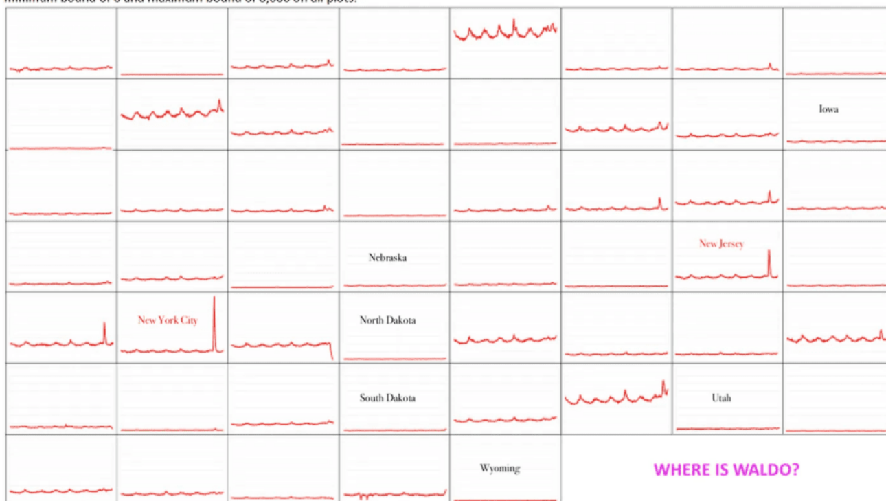
Graph 16: All Cause Deaths per Week and U.S. Jurisdiction, from MMWR week ending 1/11/2014 to MMWR week ending 11/14/2020. Vertical axis scaled with minimum bound of 0 and maximum bound of 8,000 on all plots.
